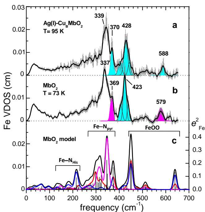
Fig. 2 The Fe VDOS determined from NRVS measurements on (a) Ag(I)–Cu B MbO 2 and (b) horse MbO 2 completely describe vibrational motion of Fe in each molecule. Shading indicates areas determined by curve fitting the VDOS, in cyan, and estimated from 57 Fe/ 54 Fe isotope shifts, in magenta. The black trace in panel (c) shows the predicted Fe VDOS, indicating regions where each Fe-ligand bond contributes to the signal. Predicted contributions from motion along x (red), y (magenta), and z (blue) refer to the coordinate system in Fig. 1 where the four pyrrole nitrogens define the xy plane and the FeOO group defines the xz plane.
