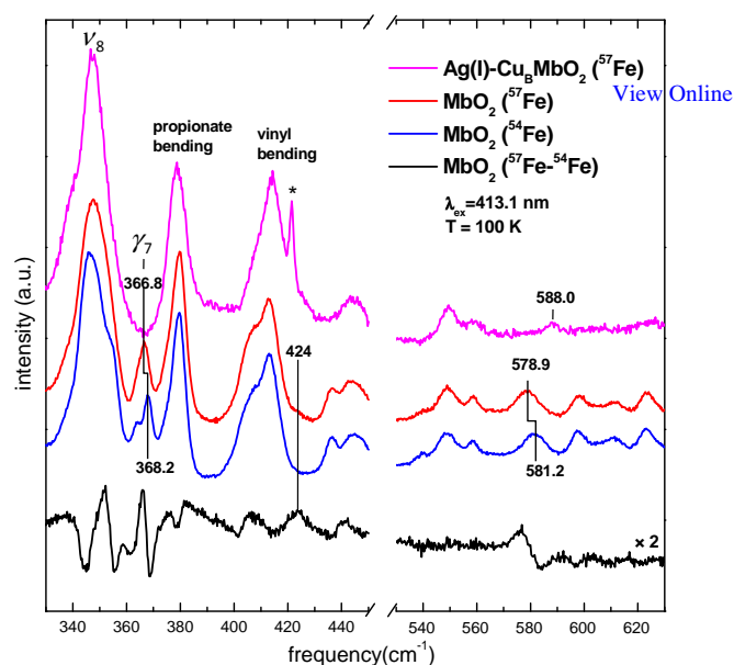
Fig. 3 Cryogenic Raman spectra recorded in resonance with the Soret absorption band include contributions from Fe vibrations, highlighted by the 57 Fe/ 54 Fe difference spectrum, among more strongly enhanced porphyrin vibrations.
