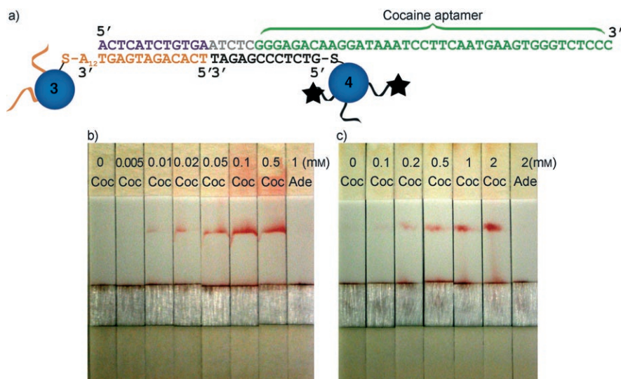
Figure 3. Lateral flow based detection of cocaine. a) DNA sequences and linkages in cocaine aptamer-linked nanoparticle aggregates. Test of the cocaine-sensing lateral flow device with varying concentrations of cocaine in buffer solution (b) and in undiluted human blood serum (c). Coc = cocaine, Ade = adenosine.
